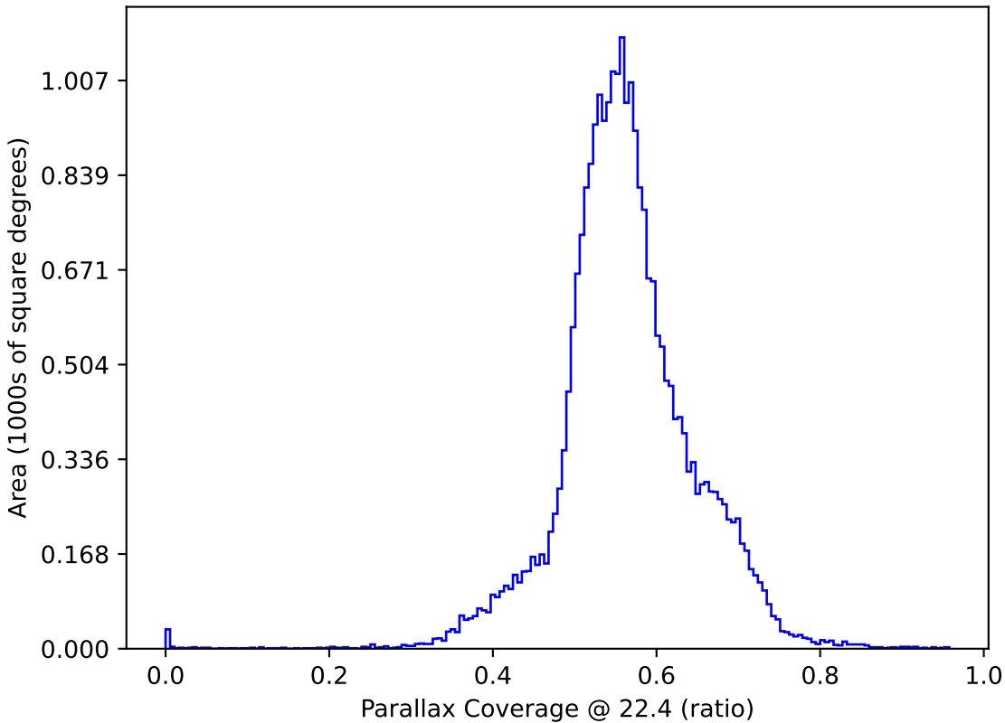
too_combined_s0.5_v3.4_10yrs : Parallax Coverage @ 22.4
