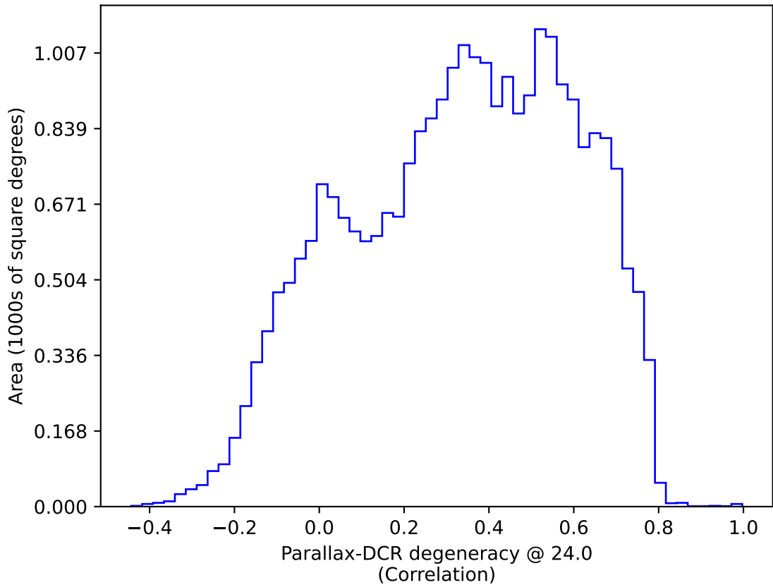
too_combined_s0.5_v3.4_10yrs : Parallax-DCR degeneracy @ 24.0
