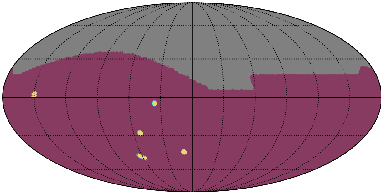
too_combined_s0.5_v3.4_10yrs : NumberOfQuickRevisits
