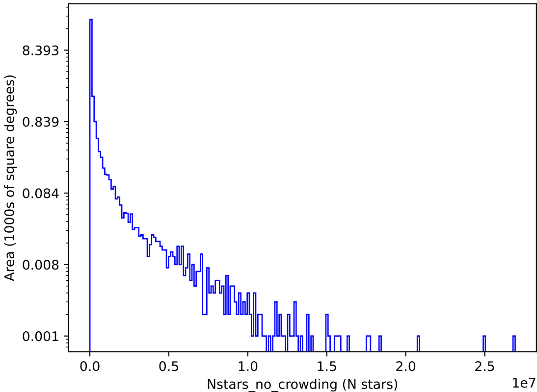
too_combined_s0.5_v3.4_10yrs z: Nstars_no_crowding
