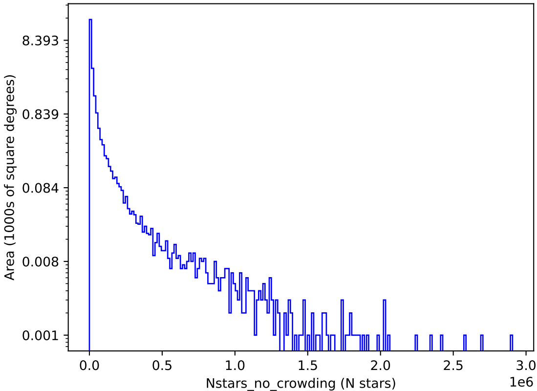
too_combined_s0.5_v3.4_10yrs u: Nstars_no_crowding
