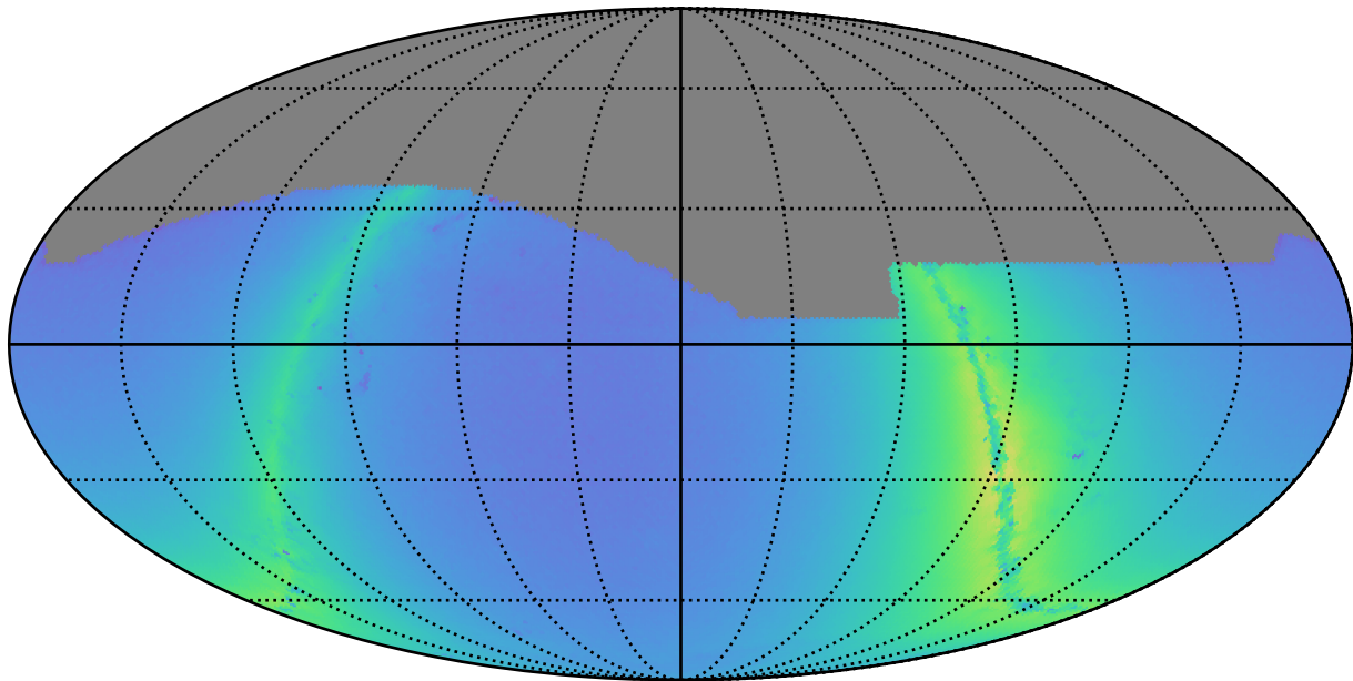
too_combined_s0.5_v3.4_10yrs r: Nstars_no_crowding
