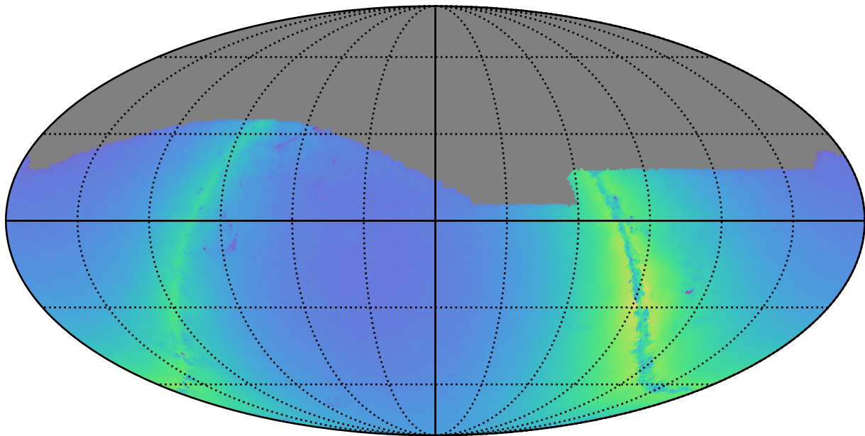
too_combined_s0.5_v3.4_10yrs g: Nstars_no_crowding
