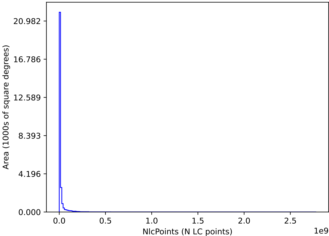
too_combined_s0.5_v3.4_10yrs : NlcPoints
