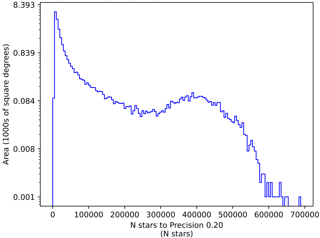
too_combined_s0.5_v3.4_10yrs z: N stars to Precision 0.20
