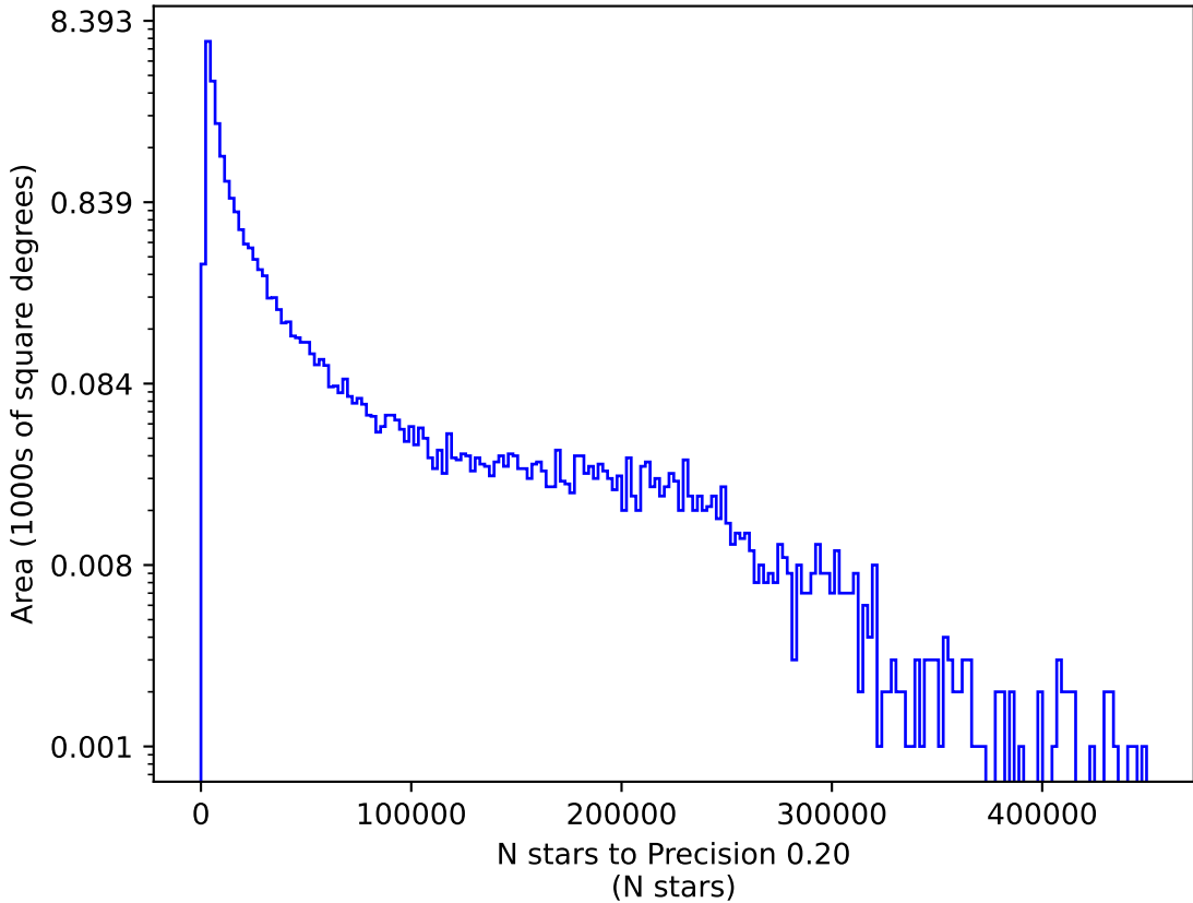
too_combined_s0.5_v3.4_10yrs u: N stars to Precision 0.20
