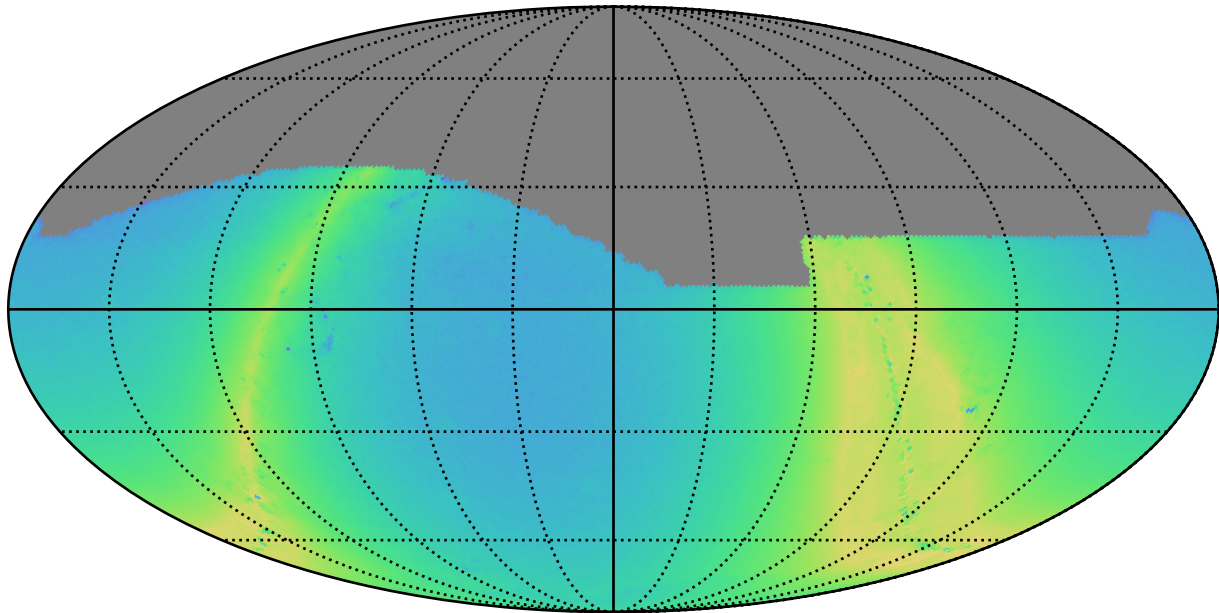
too_combined_s0.5_v3.4_10yrs r: N stars to Precision 0.20
