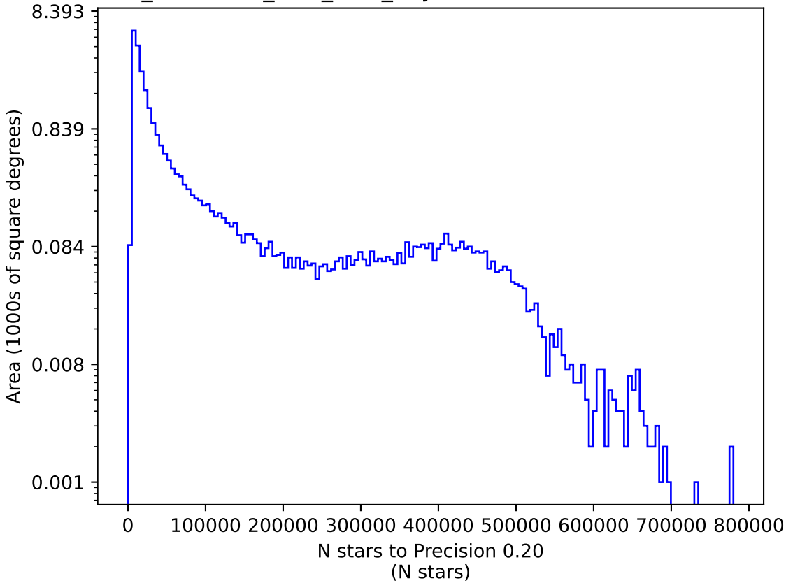
too_combined_s0.5_v3.4_10yrs i: N stars to Precision 0.20
