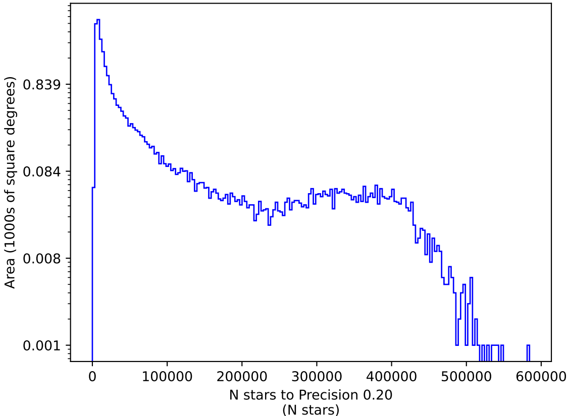
too_combined_s0.5_v3.4_10yrs g: N stars to Precision 0.20
