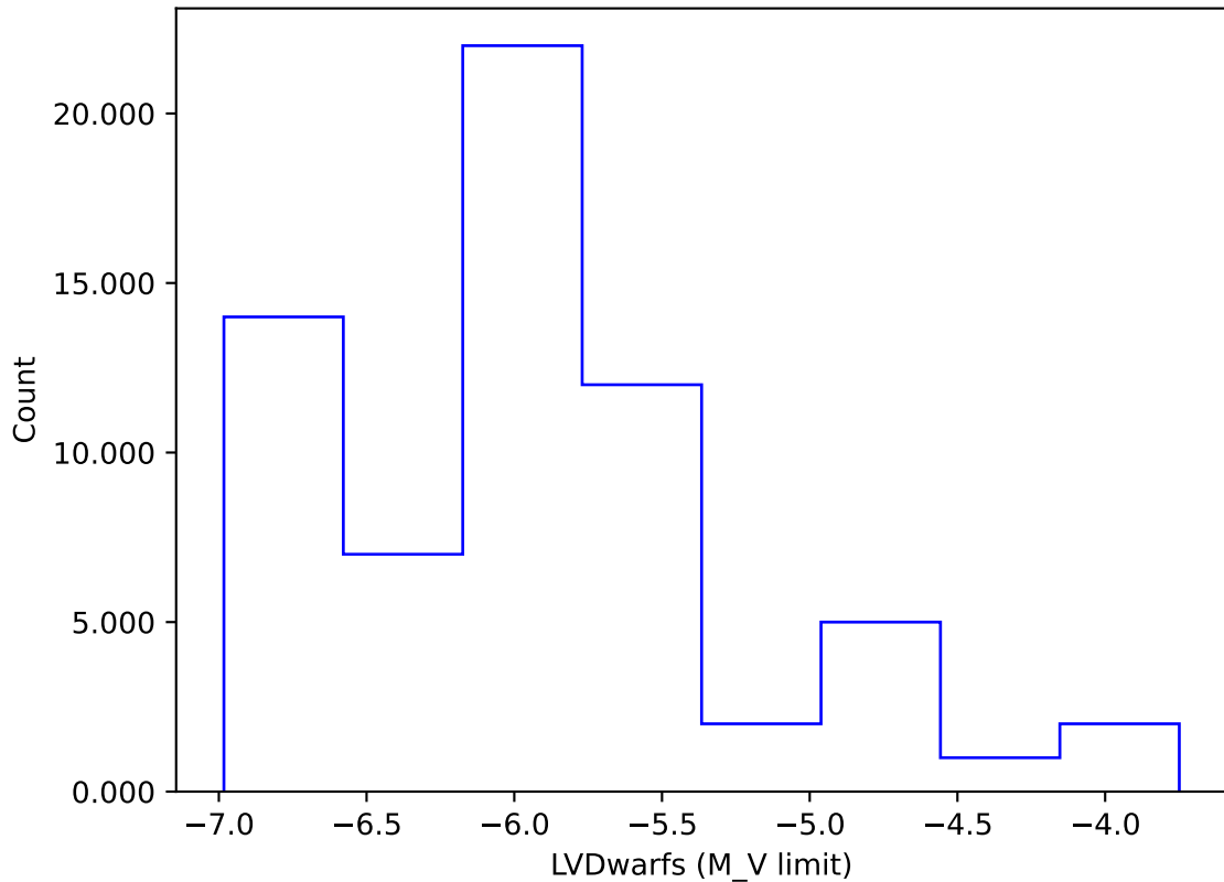
too_combined_s0.5_v3.4_10yrs gi: LVDwarfs
