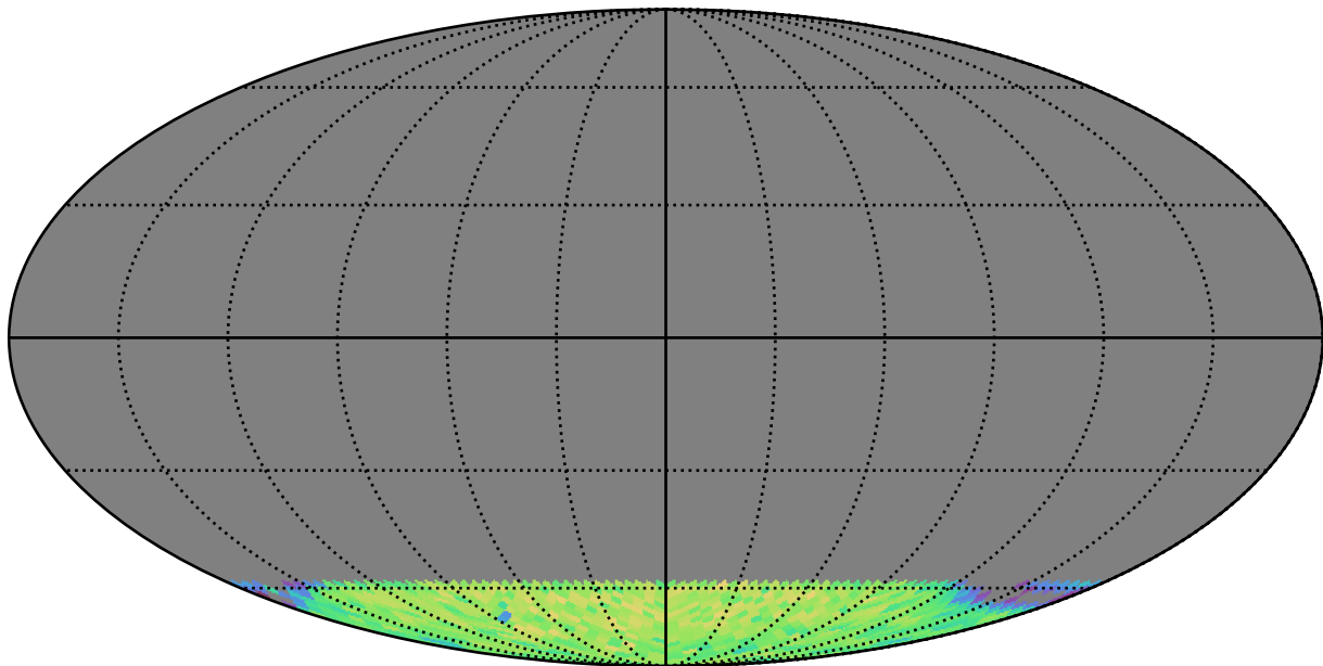
too_combined_s0.5_v3.4_10yrs gi SCP: LVDwarfs
