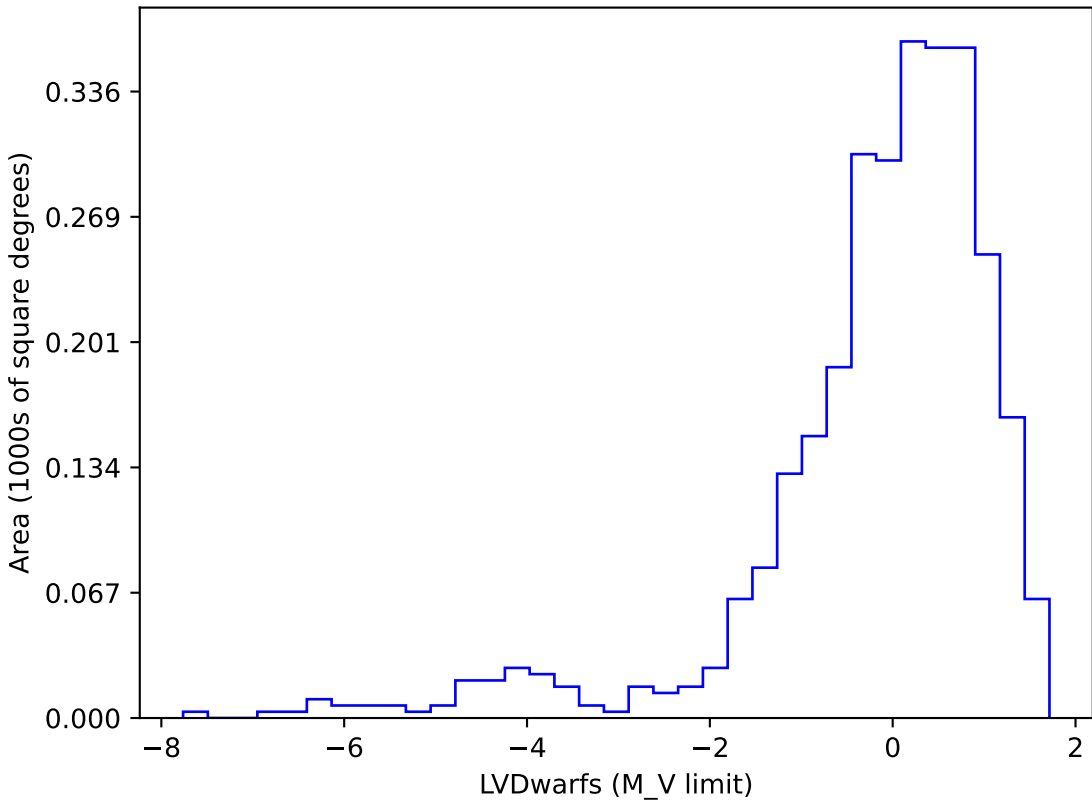
too_combined_s0.5_v3.4_10yrs gi SCP: LVDwarfs
