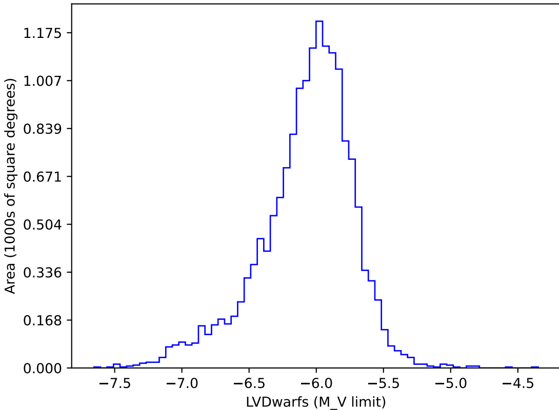
too_combined_s0.5_v3.4_10yrs gi: LVDwarfs
