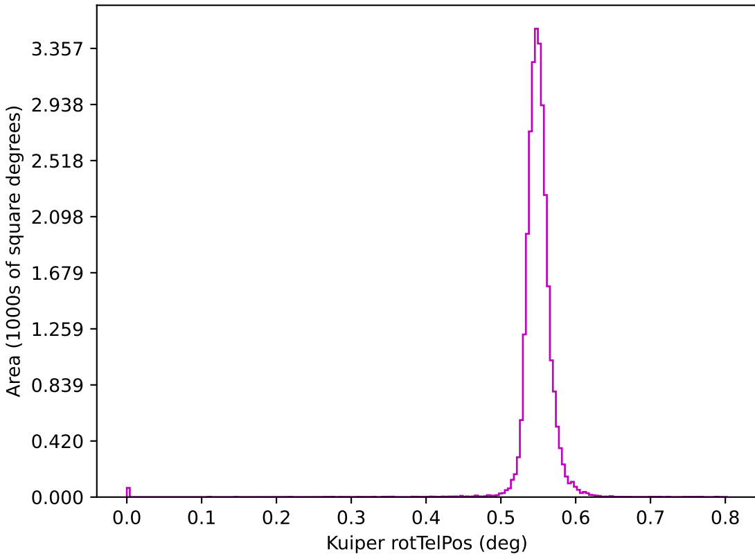
too_combined_s0.5_v3.4_10yrs z: Kuiper rotTelPos
