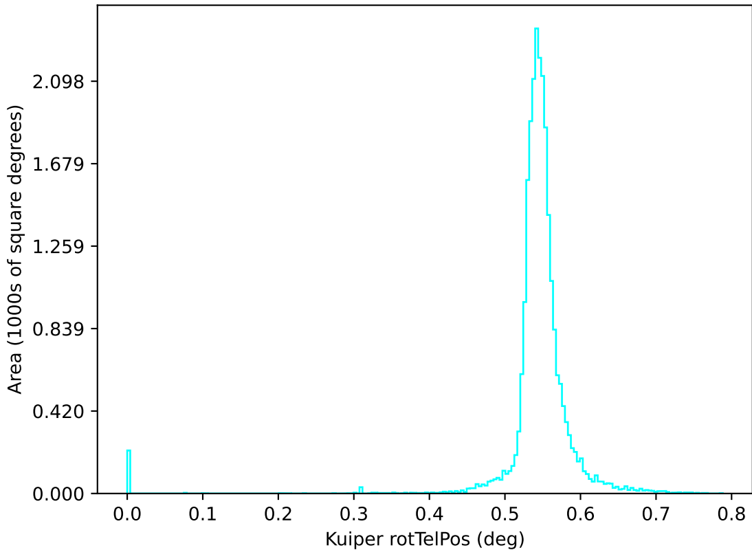
too_combined_s0.5_v3.4_10yrs u: Kuiper rotTelPos
