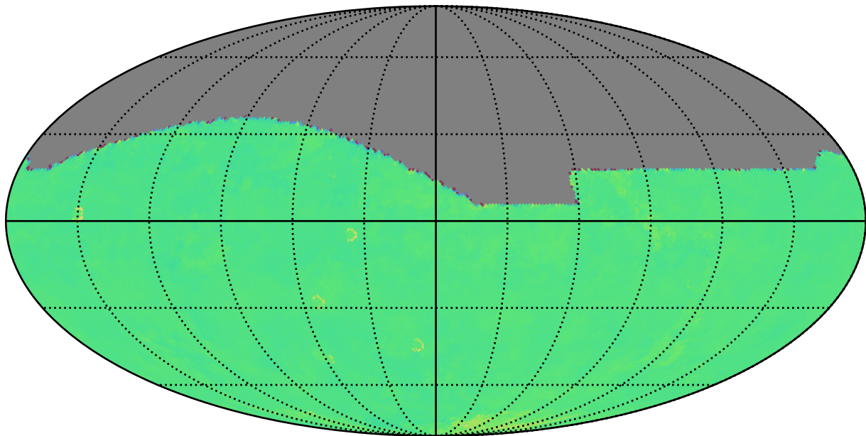
too_combined_s0.5_v3.4_10yrs r: Kuiper rotTelPos
