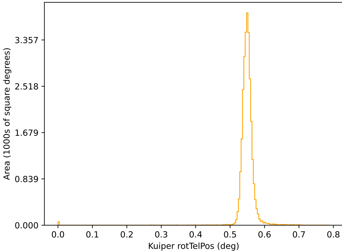
too_combined_s0.5_v3.4_10yrs r: Kuiper rotTelPos
