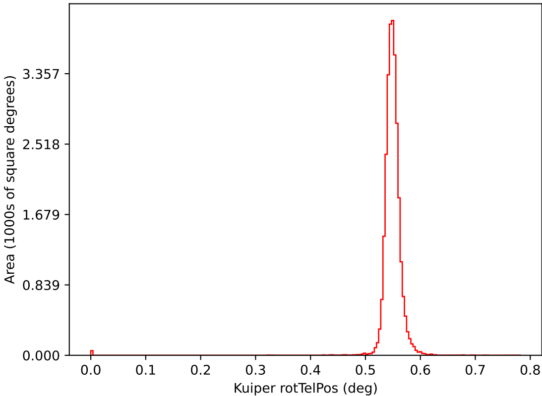
too_combined_s0.5_v3.4_10yrs i: Kuiper rotTelPos
