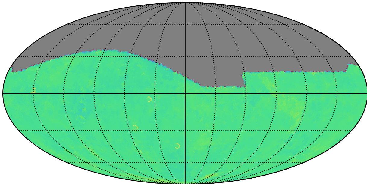
too_combined_s0.5_v3.4_10yrs g: Kuiper rotTelPos
