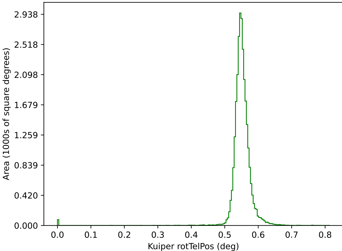
too_combined_s0.5_v3.4_10yrs g: Kuiper rotTelPos
