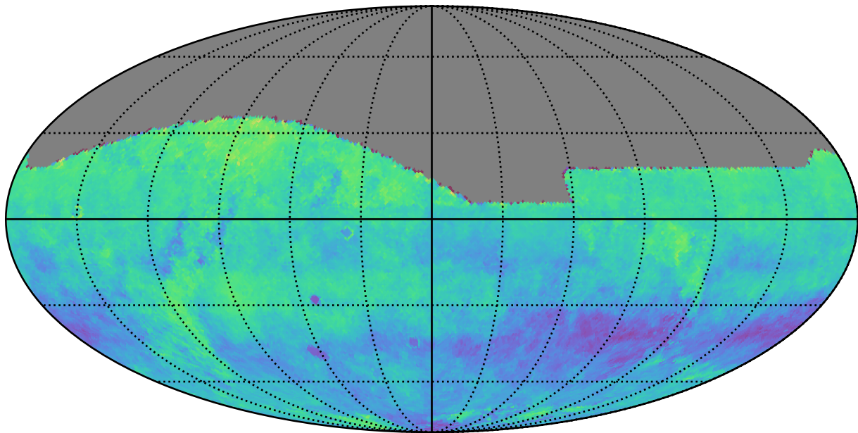
too_combined_s0.5_v3.4_10yrs z: Kuiper rotSkyPos
