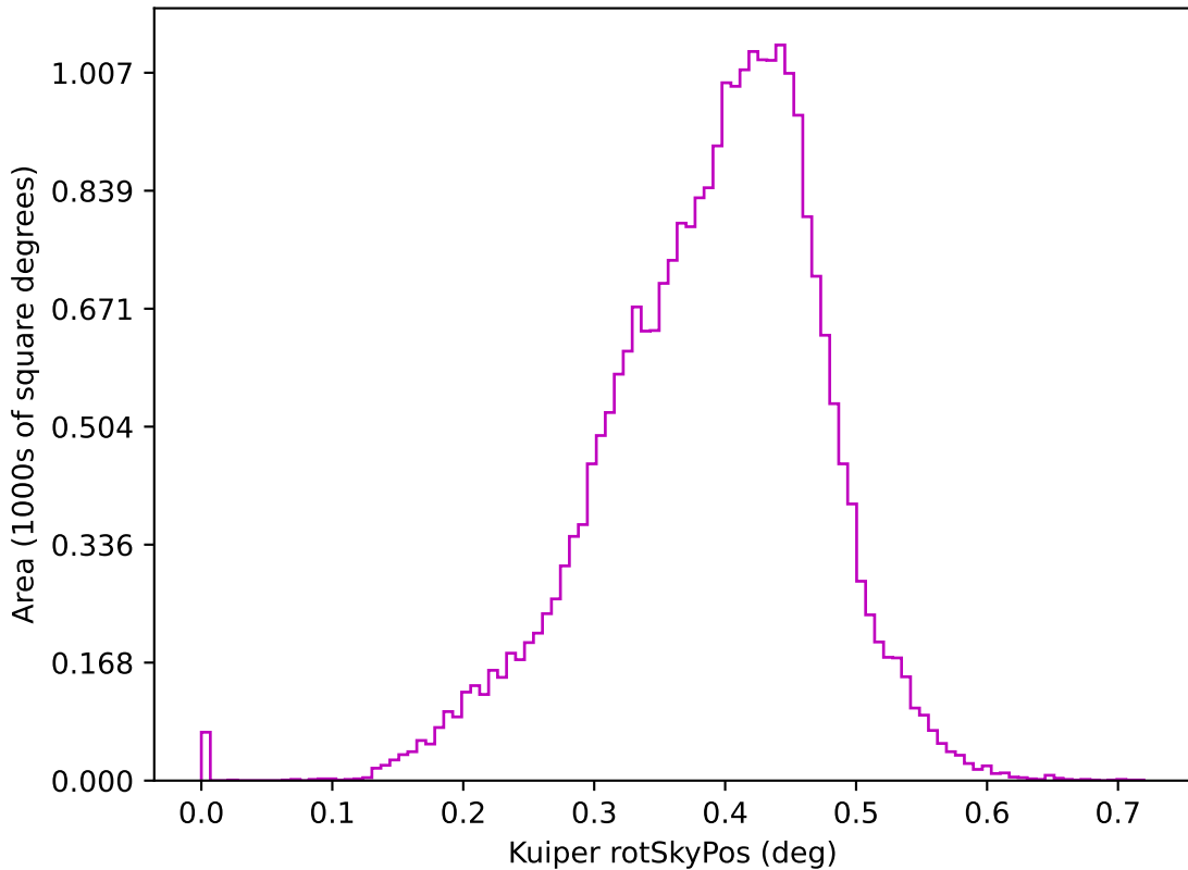
too_combined_s0.5_v3.4_10yrs z: Kuiper rotSkyPos
