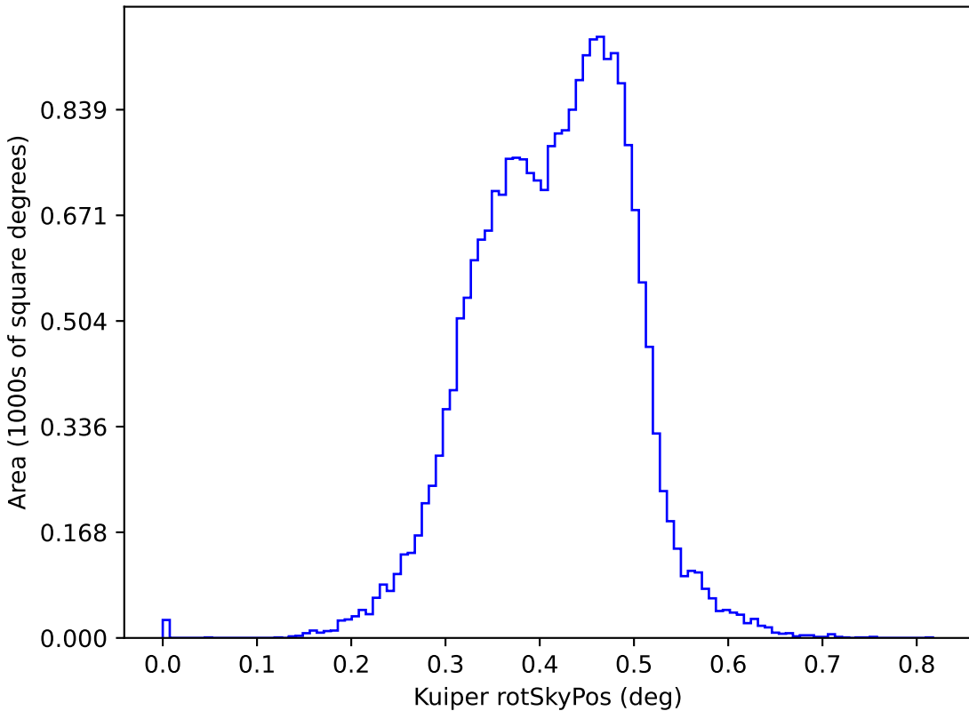
too_combined_s0.5_v3.4_10yrs y: Kuiper rotSkyPos
