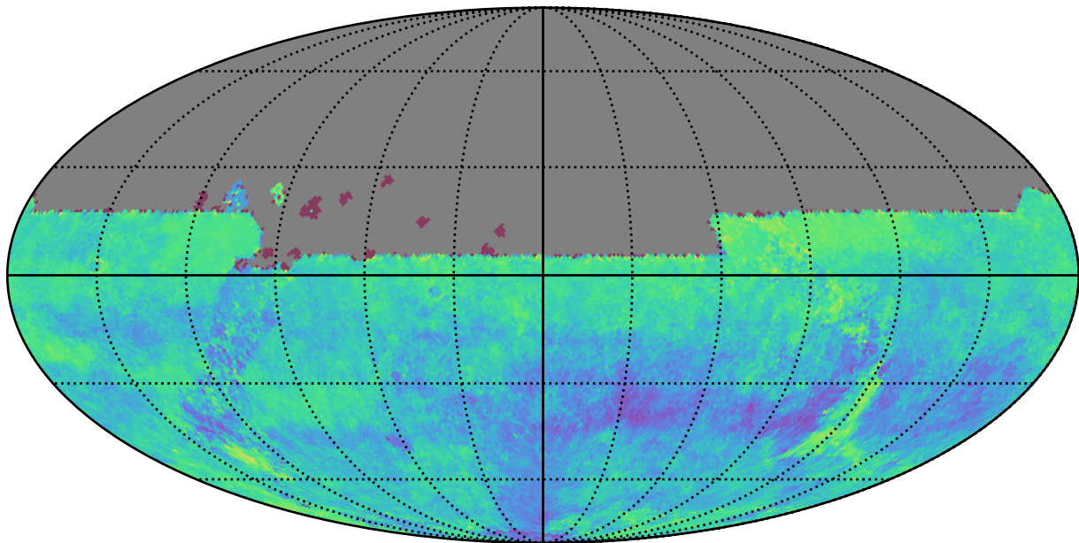
too_combined_s0.5_v3.4_10yrs u: Kuiper rotSkyPos
