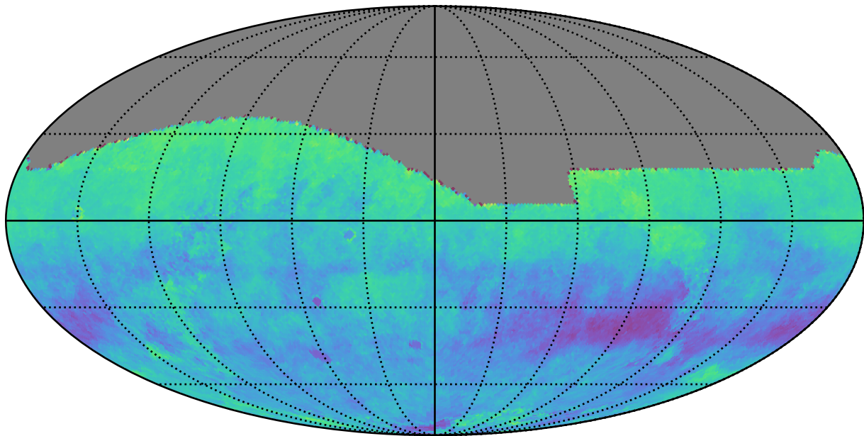
too_combined_s0.5_v3.4_10yrs r: Kuiper rotSkyPos
