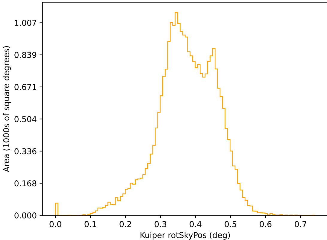
too_combined_s0.5_v3.4_10yrs r: Kuiper rotSkyPos
