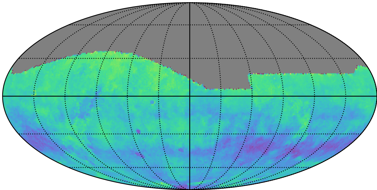
too_combined_s0.5_v3.4_10yrs i: Kuiper rotSkyPos
