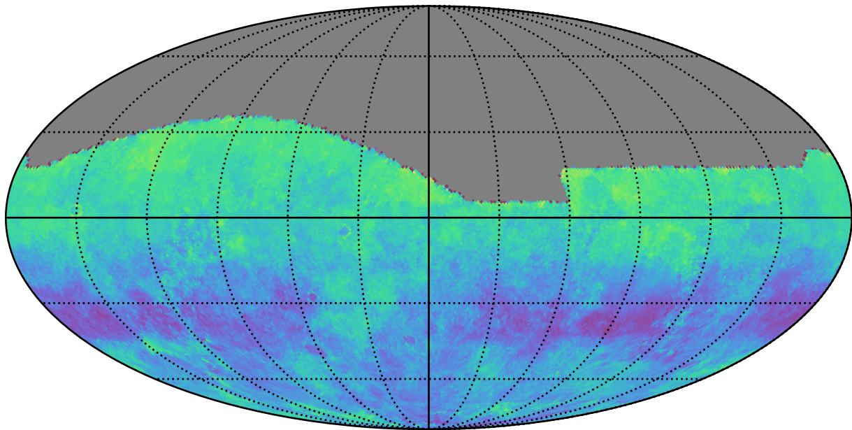
too_combined_s0.5_v3.4_10yrs g: Kuiper rotSkyPos
