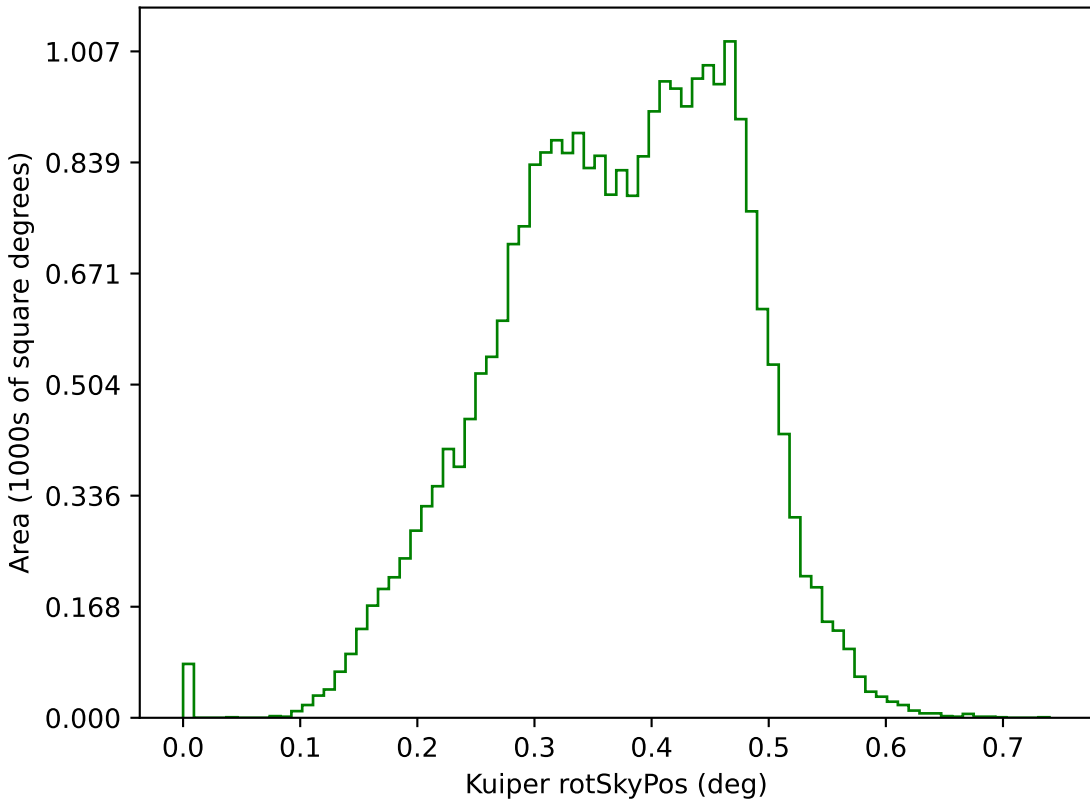
too_combined_s0.5_v3.4_10yrs g: Kuiper rotSkyPos
