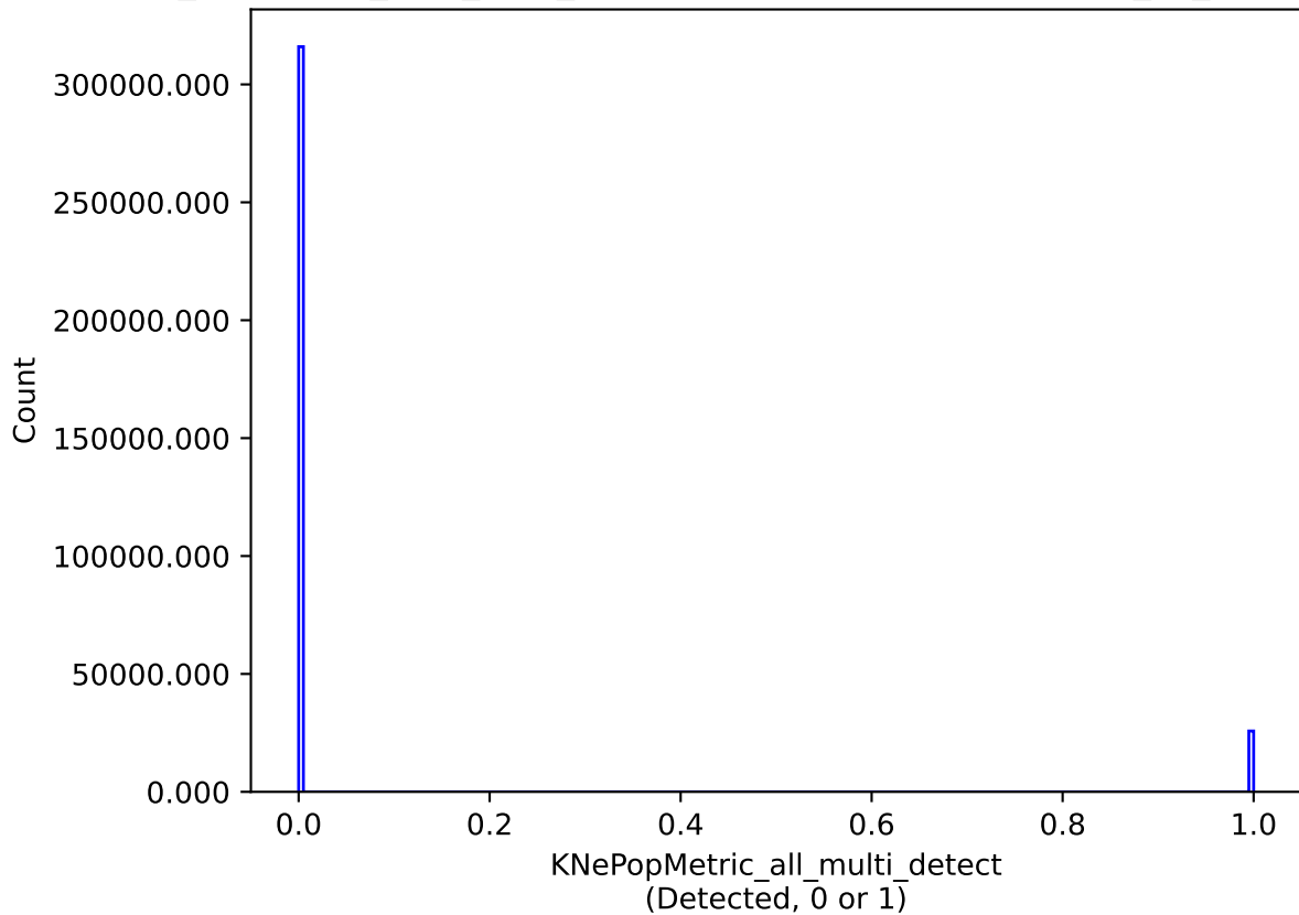
too_combined_s0.5_v3.4_10yrs all models: KNePopMetric_all_multi_detect
