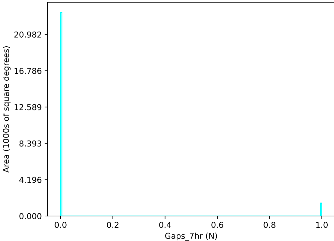
too_combined_s0.5_v3.4_10yrs u band: Gaps_7hr
