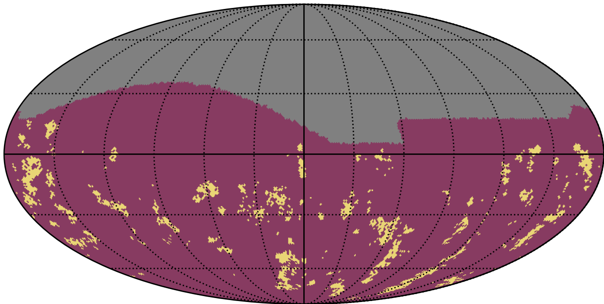
too_combined_s0.5_v3.4_10yrs g band: Gaps_7hr
