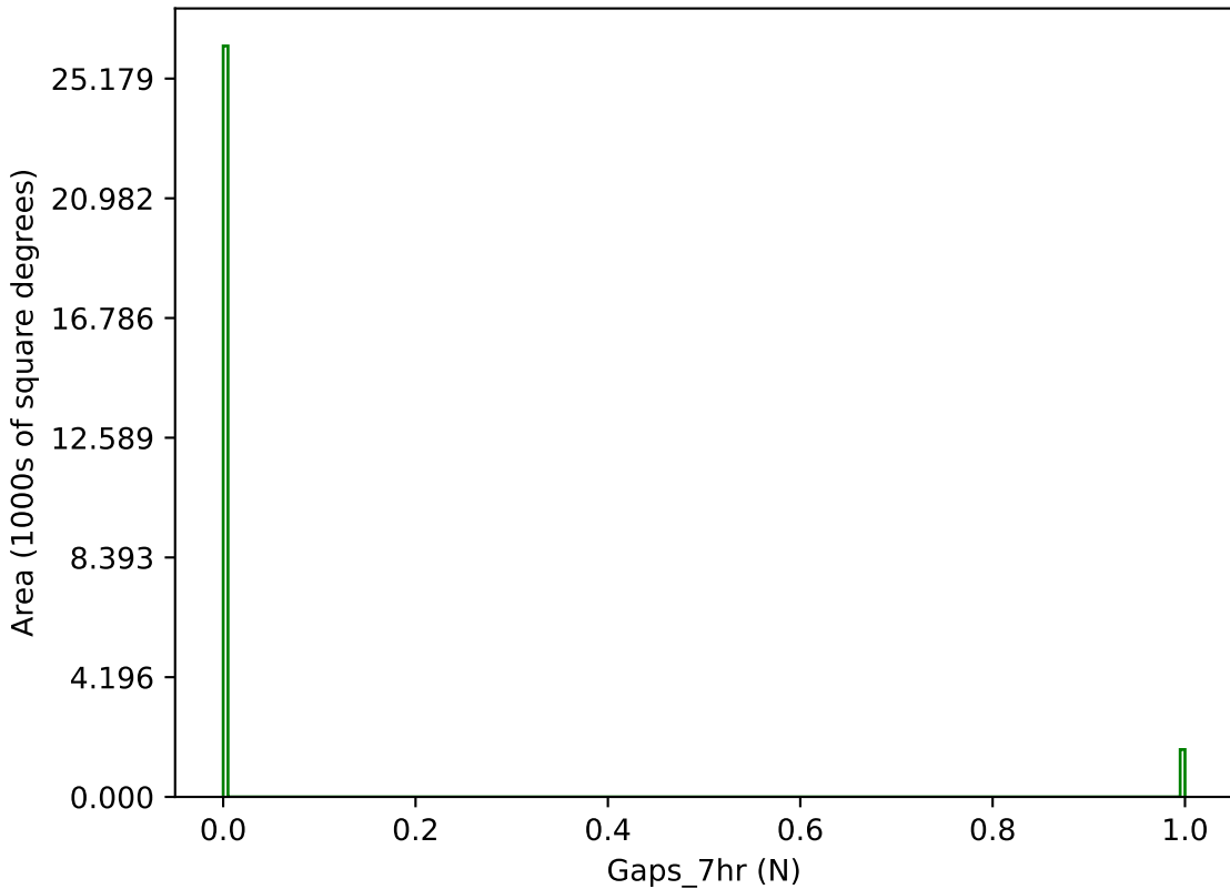
too_combined_s0.5_v3.4_10yrs g band: Gaps_7hr
