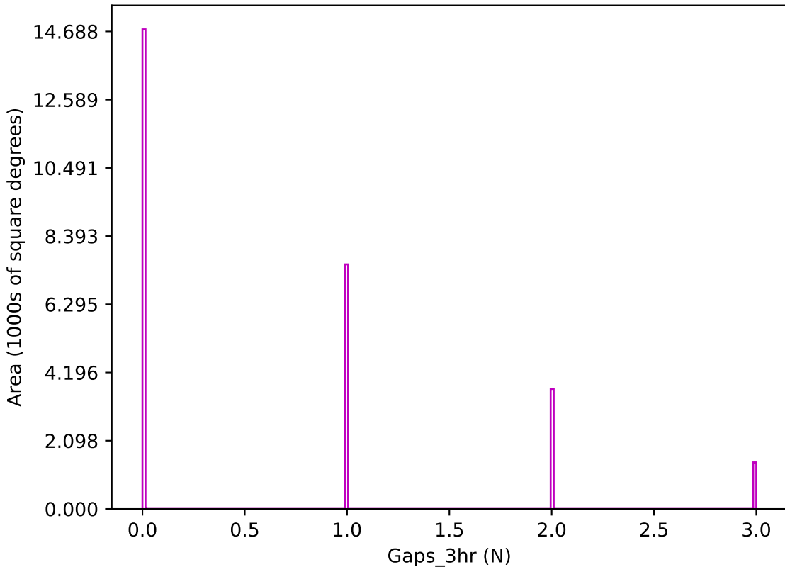
too_combined_s0.5_v3.4_10yrs z band: Gaps_3hr
