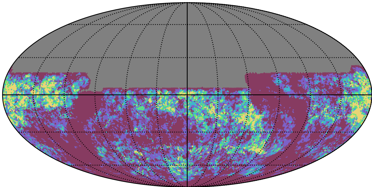
too_combined_s0.5_v3.4_10yrs y band: Gaps_3hr
