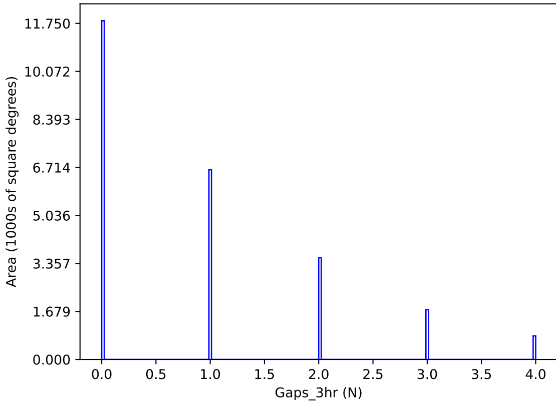
too_combined_s0.5_v3.4_10yrs y band: Gaps_3hr
