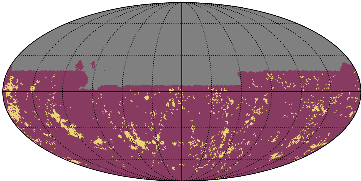
too_combined_s0.5_v3.4_10yrs u band: Gaps_3hr
