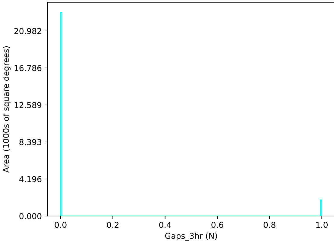
too_combined_s0.5_v3.4_10yrs u band: Gaps_3hr
