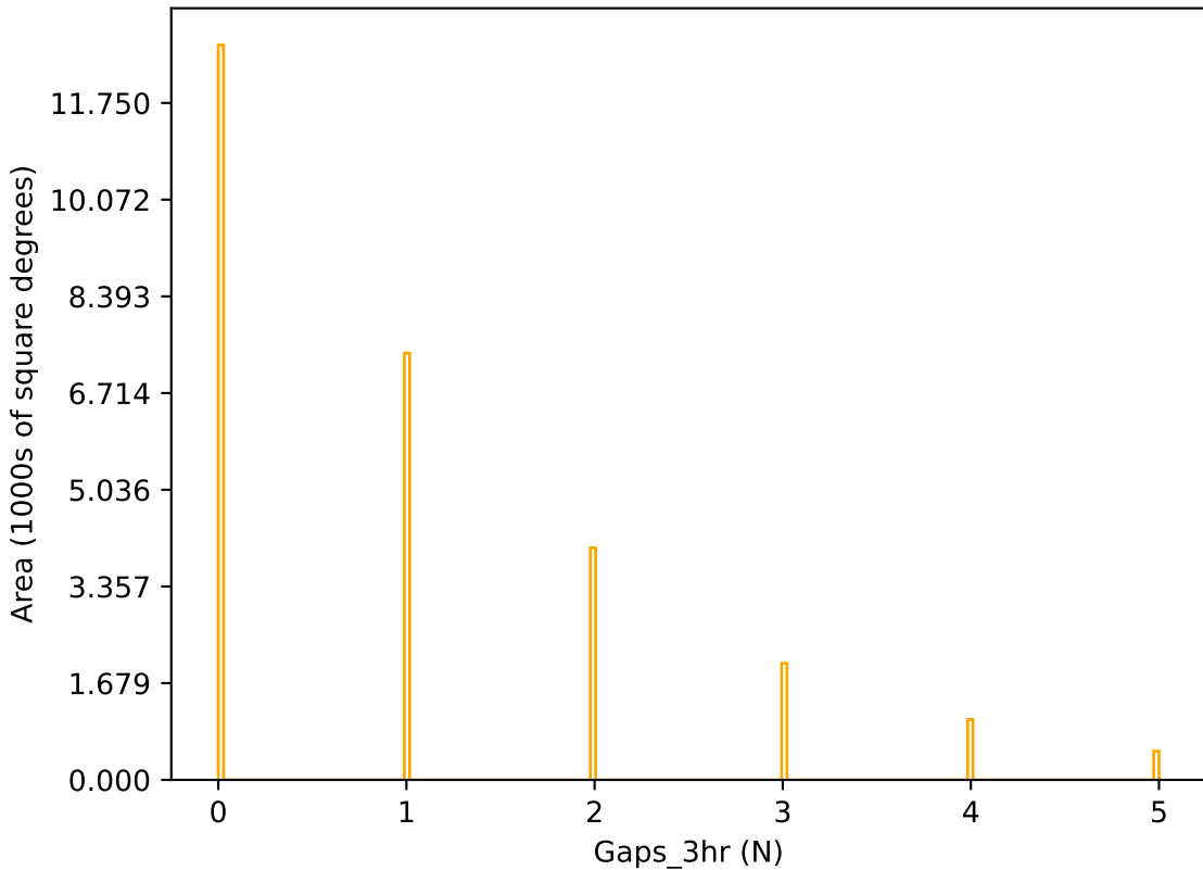
too_combined_s0.5_v3.4_10yrs r band: Gaps_3hr
