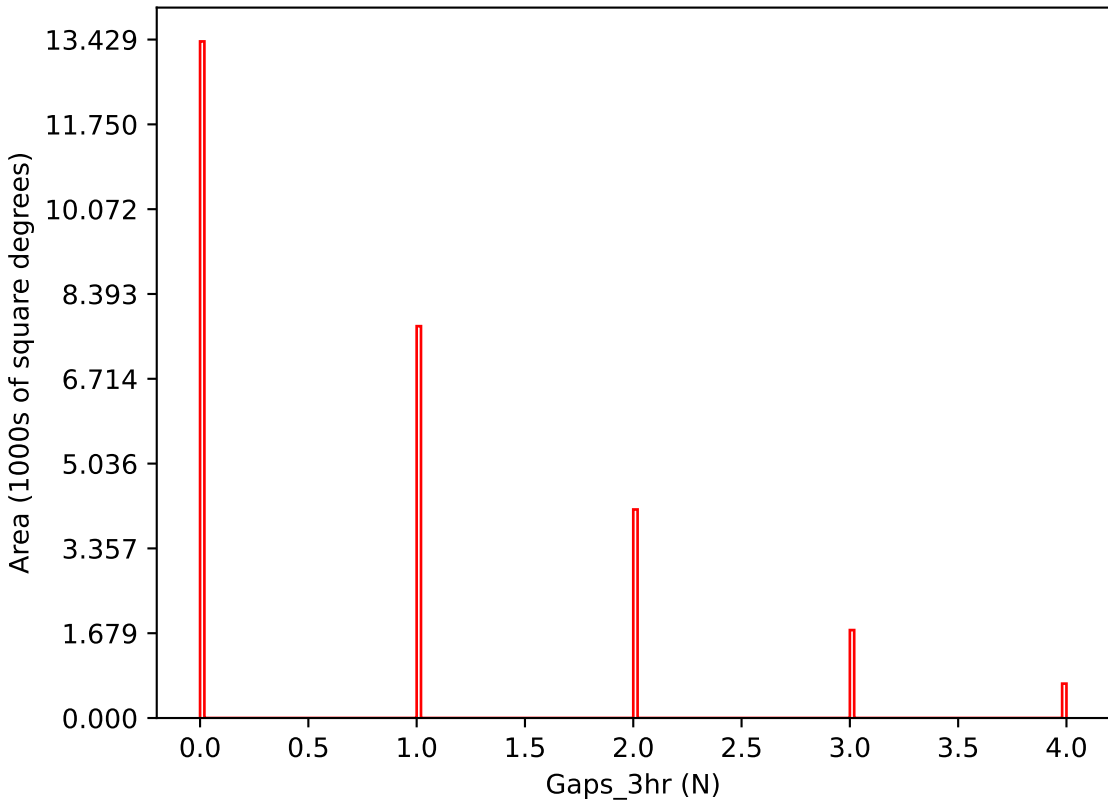
too_combined_s0.5_v3.4_10yrs i band: Gaps_3hr
