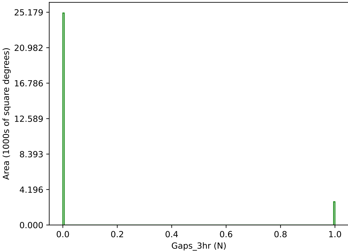
too_combined_s0.5_v3.4_10yrs g band: Gaps_3hr
