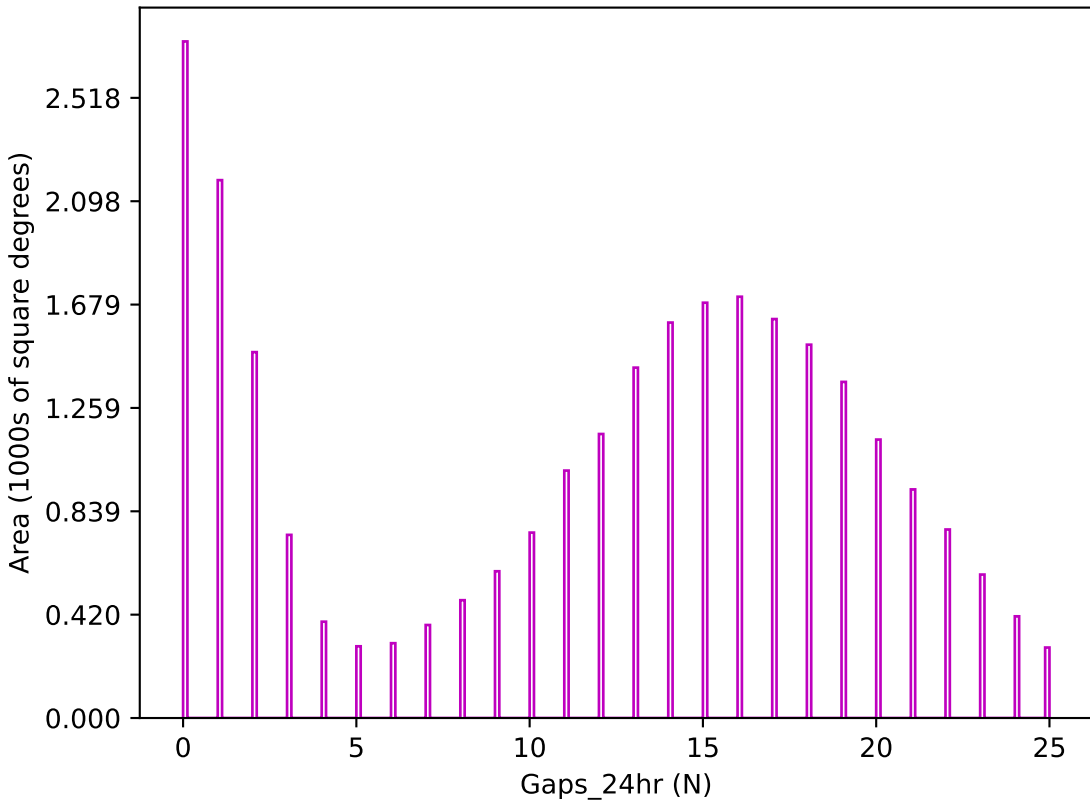
too_combined_s0.5_v3.4_10yrs z band: Gaps_24hr
