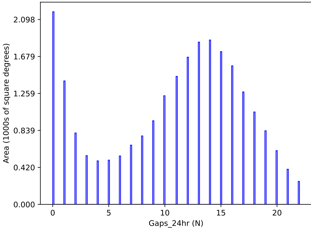
too_combined_s0.5_v3.4_10yrs y band: Gaps_24hr
