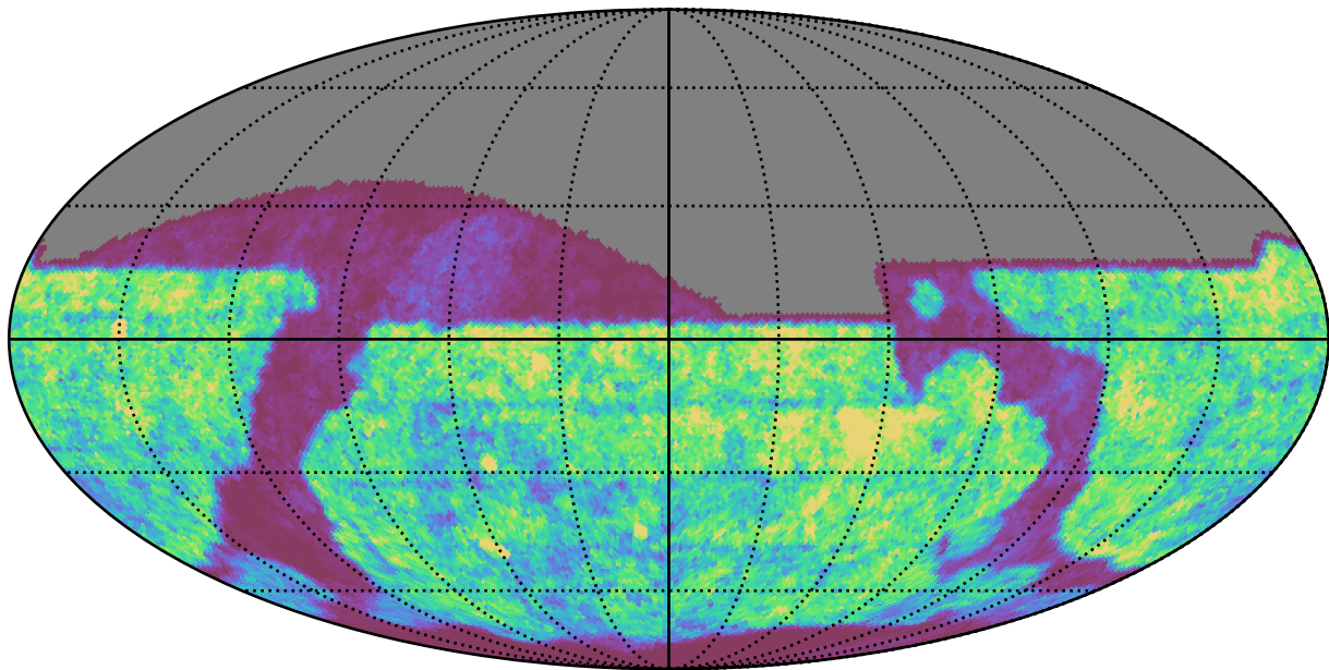
too_combined_s0.5_v3.4_10yrs r band: Gaps_24hr
