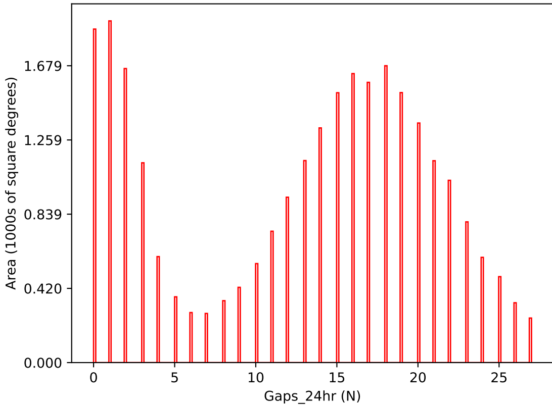
too_combined_s0.5_v3.4_10yrs i band: Gaps_24hr
