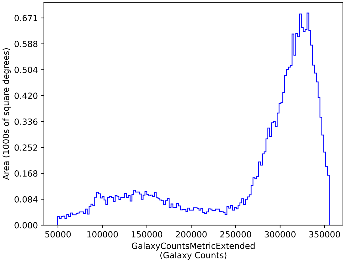
too_combined_s0.5_v3.4_10yrs y: GalaxyCountsMetricExtended
